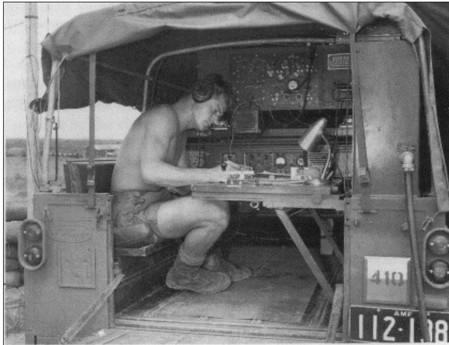
Photo 2.8 - Cpl Rex Gabel, 709 Signal Troop, transmits in morse code at Bien Hoa to HQ AAFV in Saigon. The radio set in use is the medium-power AN/TRC-75 (Sept 1965)
